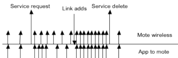
Figure 1. The sequence of packets through a burst period for a mote. Prior to the burst the mote is able to transmit packets as quickly as the application can hand them over. When the burst mode begins, the mote starts to NACK the application which needs to throttle in response. After the mote gets new links in response to the service request, the application can send the burst packets as quickly as it can generate them.
