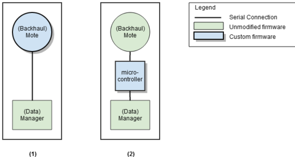
Figure 3 - Setups for the backhaul bridge.
