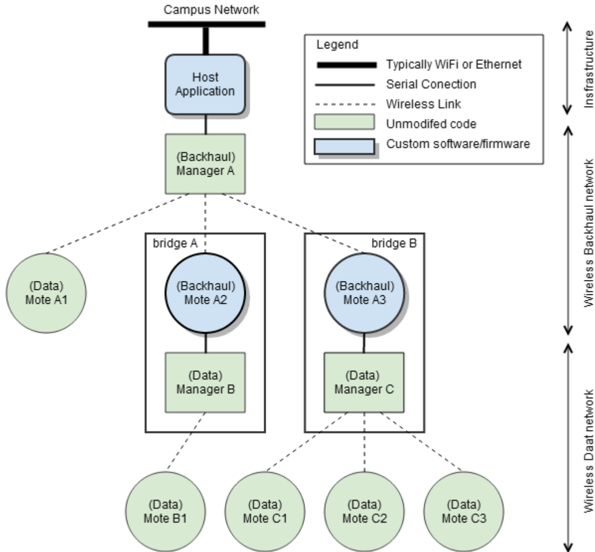
Figure 2 - A Mesh-of-Meshes deployment.
