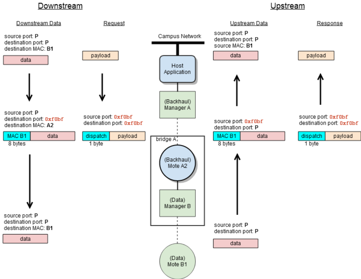
Figure 4 - The different flows handled by the tunneling protocol.
