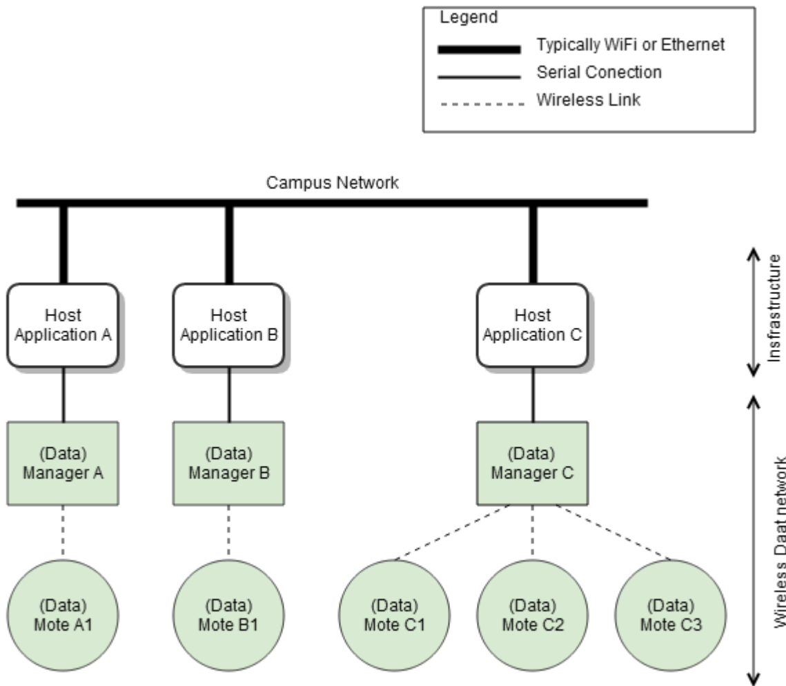
Figure 1 - A deployment with several independent wireless data networks.
